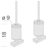
2518 Simple suspension
