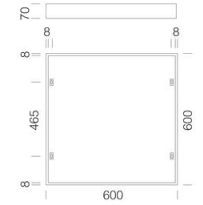
595 Frame 600x600 h 70 mm
