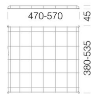
36 Protection grid
