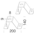
39 Ceiling bracket
