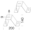
39 Ceiling bracket
