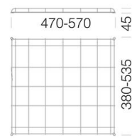
36 Protection grid
