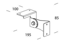
537 Adjustable bracket
